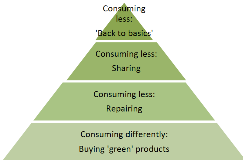
Figure 1: The Resource-Consumption-Hierarchy
